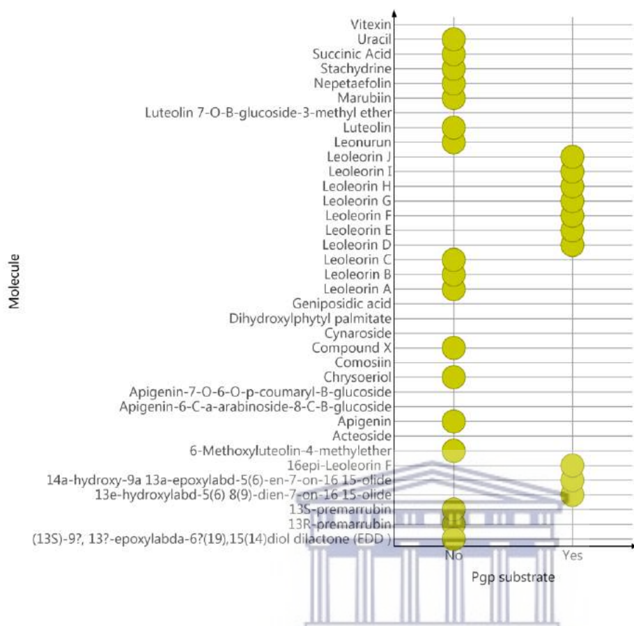
Figure 3.10: Illustration showing the possibility of the 36 compounds from L. leonurus being P-gp substrates.
