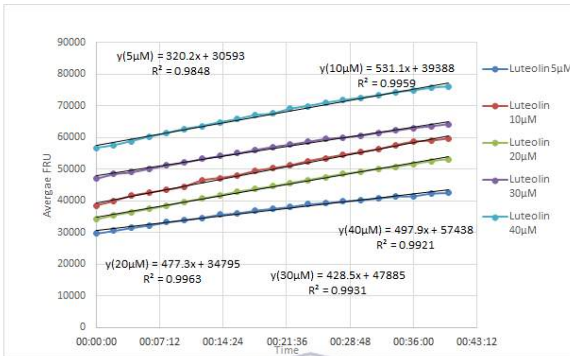
Figure 5.8: Inhibition of fluorescence produced by MAO-B - catalysed cleavage of tyramine, by luteolin (5µM, 10µM, 20µM, 30µM and 40µM).
