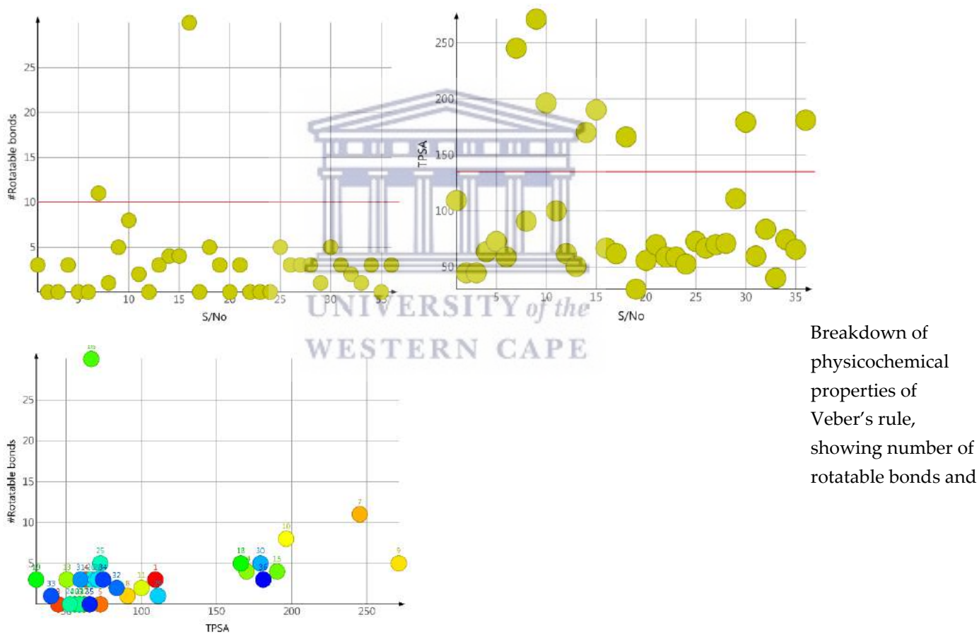
Figure 3.7: Graphs showing breakdown of physicochemical properties under Veber's rule (top right and left). The red lines represent the desired ideal values for TPSA and rotatable bonds. All the compounds assessed (lower left) compounds which passed Veber's rule (lower right).
