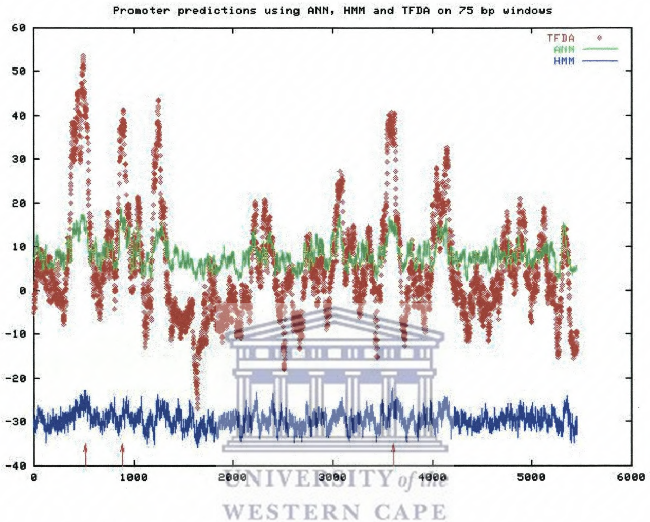
Figure 6.4. Prediction scores of NN (green), HMM (blue) and TFDA (red) on 75 bp window sized sequences covering ~5500 bp region of B.subtilis genome harboring promoters veg , sspF and spoVG . Test sequences and prediction scores were obtained by shifting each previous window by 1 bp. Results from HMM were multiplied by (0.35) to enable the values to fit onto the graphs. Promoters veg , sspF and spoVG are found in positions 520, 890 and 3606 respectively as indicated by the arrows. The individual plots for predictions of ANN, HMM and TFDA can be found in Appendix_twentythree, Appendix_twentyfour and Appendix_twentyfive respectively.
