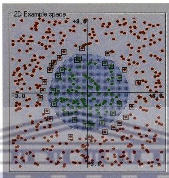
Figure 2.8: The non-linear SVM classification with RBF kernel
