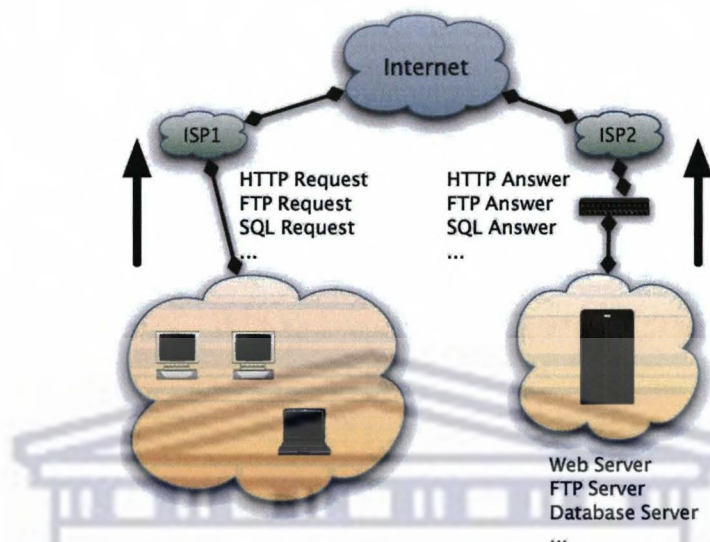
Figure 4.1: One server serves users with different requirements
