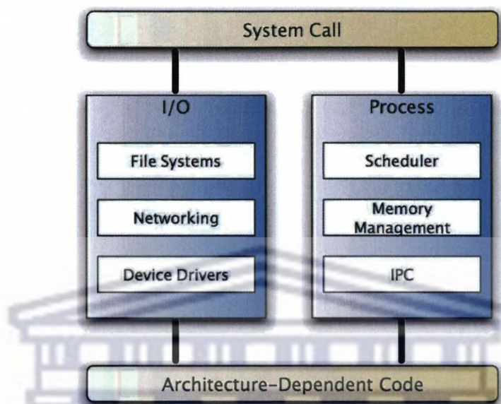
Figure 3.2: The components of the kernel
