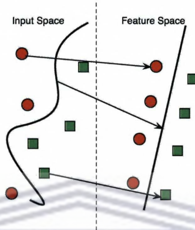
Figure 2.2: Mapping from input space to feature space
