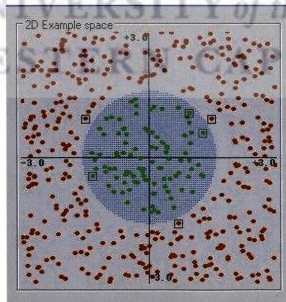
Figure 2.7: The non-linear SVM classification with polynomial kernel
