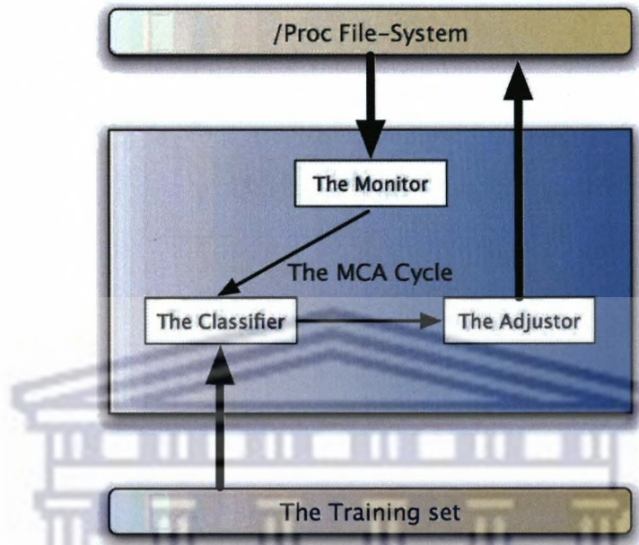
Figure 5.1: Overview of KernTune
