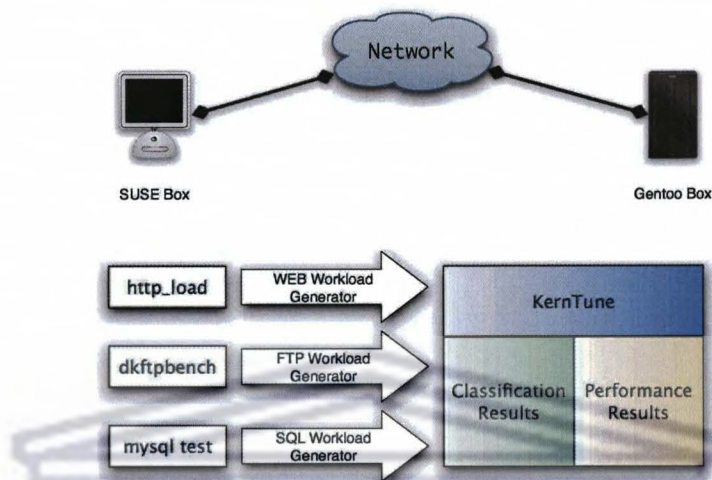
Figure 6.1: KernTune Test Bed
