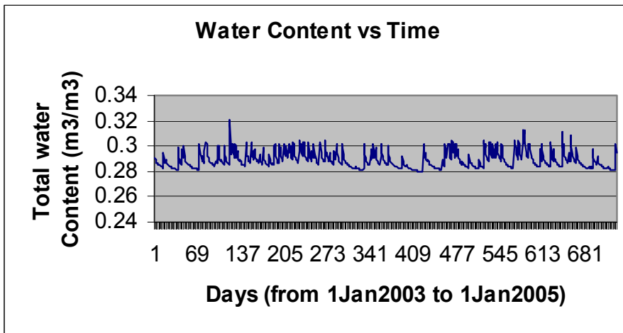
Figure 6.4: Water content vs time for topsoil, Berg river site 1 using Macro 5.0
