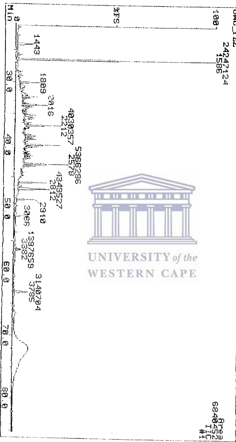
Figure 4.6. Gas chromatogram of the active compound after 90 minutes
