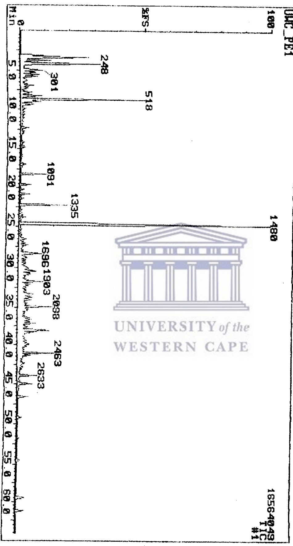
Figure 4.5. Gas chromatogram of active compound after 60 minutes
